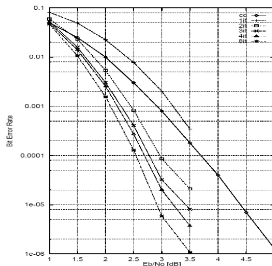
Figure 3.1: BER for rate 1/2 turbo codes, 200 bit interleaver, QPSK modulation, AWGN channel.
